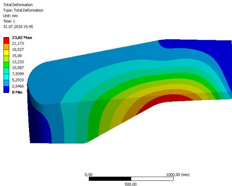
Fig. 8. Displacement field, mm
