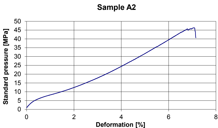
Fig. 7. "Strain-stress" curve of sample A2
