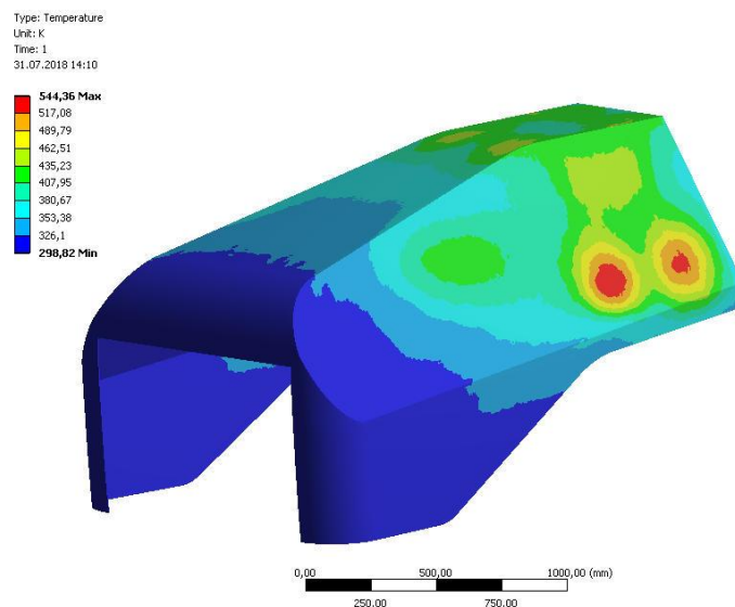
Fig. 4. Temperature field obtained for the hood
