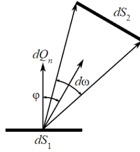
Fig. 2. Illustration of the Lambert law
