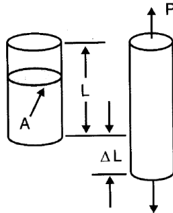
Fig. 3. Uniaxial stretching
